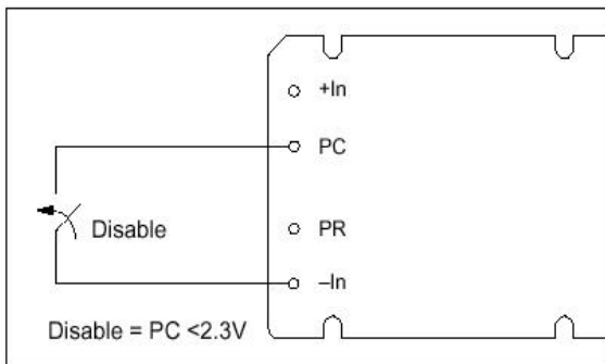
Figure 1—Module enable/disable.
