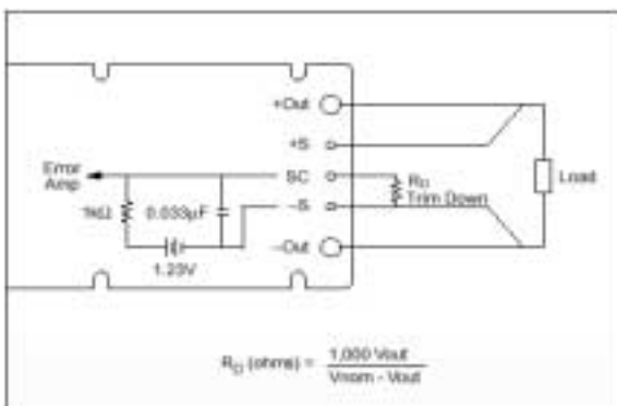
Figure 2 – Output voltage trim down circuit
