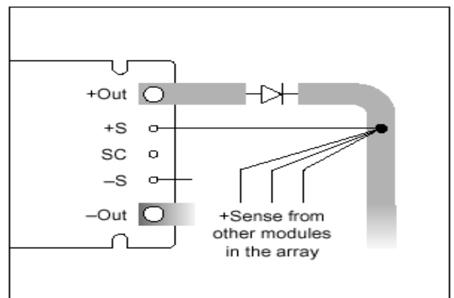
Figure 6 – OR'ing diodes connections.
