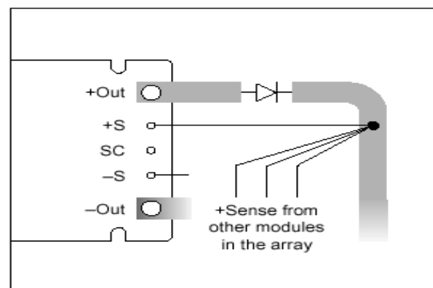
Figure 6 – OR'ing diodes connections.
