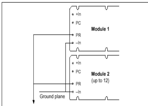
Figure 4 – DC coupled single – wire interface.
