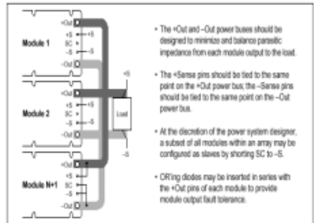
Figure 5 – N+1 module array output connections.
