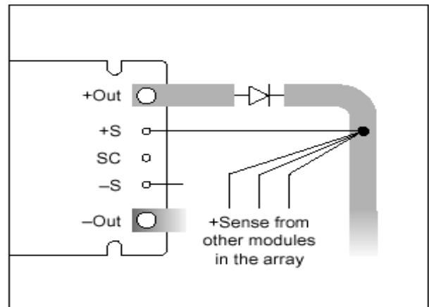
Figure 6 – OR'ing diodes connections.
