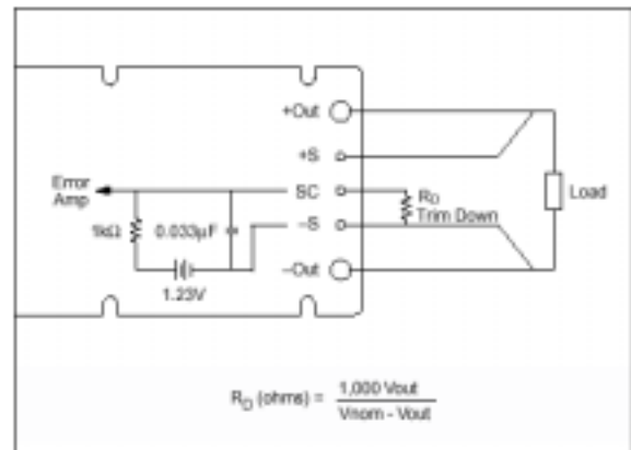
Figure 2 – Output voltage trim down circuit Trim Down
